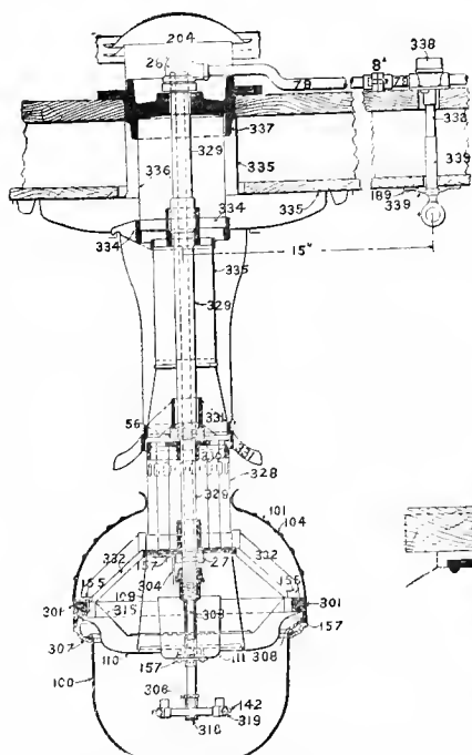
Fig. 3238. Nos. 192 and 193. SECTION CENTER-SUSPENSION LAMP. (261)
